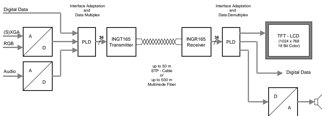
Figure 1: GigaSTaR Multimedia Link
