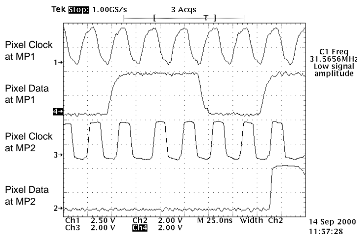
Figure 11 : Pixel Clock and Data Timing
