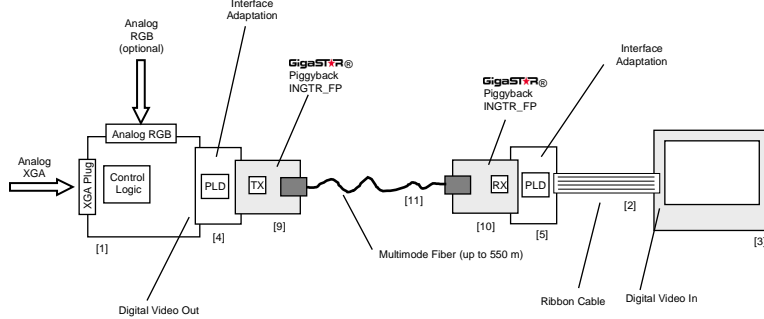
Figure 5: GigaSTaR Display Link with Multimode Fiber
